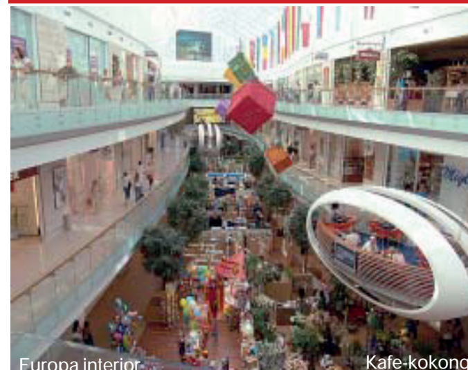
Europa interior
